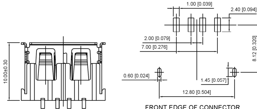
FRONT EDGE OF CONNECTOR PCB LAYOUT (T=1.60mm)
