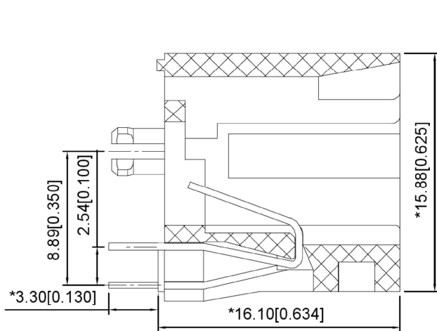
CUTAWAY VIEW
