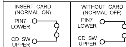
Circuit Diagram for Card Detect Switch
