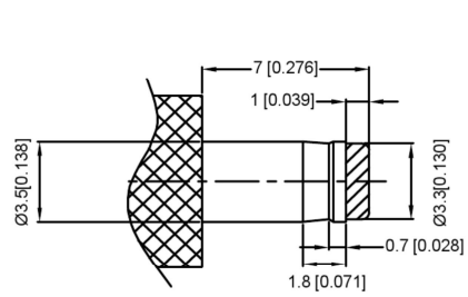
( Ø3.5mm DC PLUG DETAIL DRWING )
