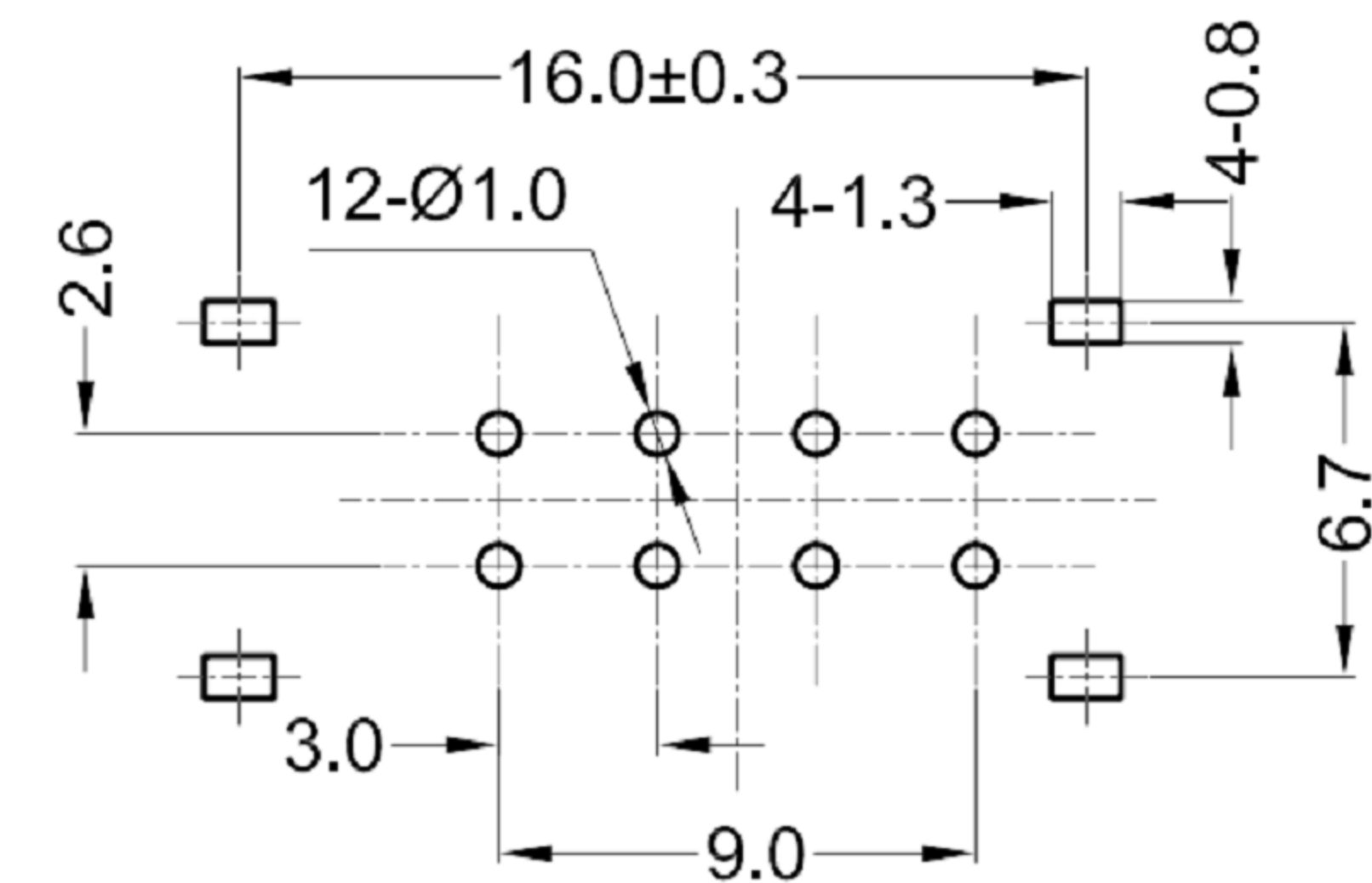
P.C.B LAYOUT BOTTOM VIEW
