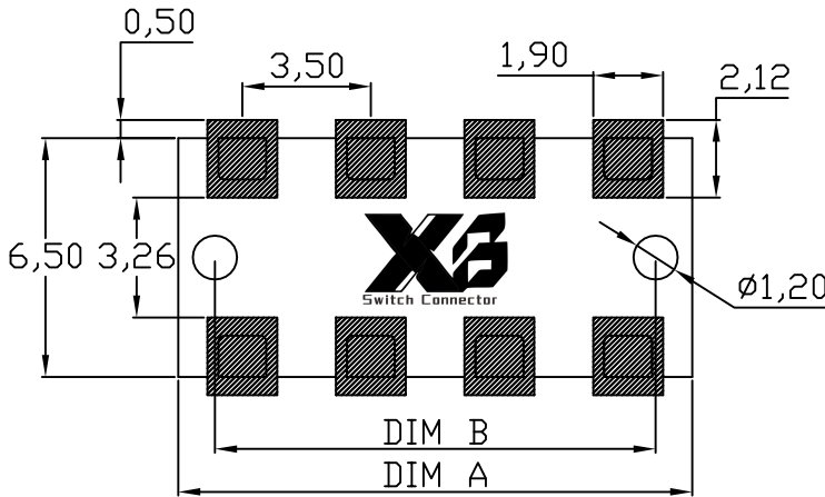
RECOMMENDED PCB LAYOUT TOP VIEW (.XX±0.05)
