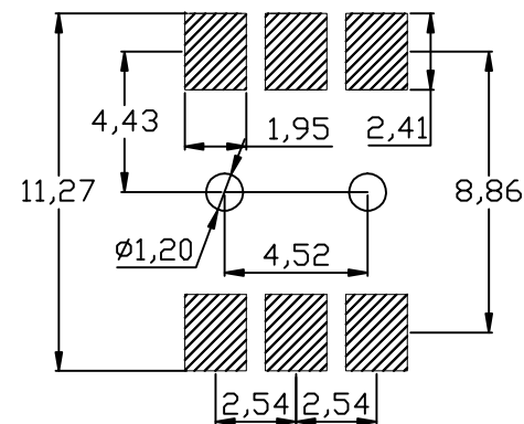
RECOMMENDED PCB LAYOUT TOP VIEW(. XX±0.05)
