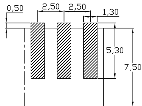
RECOMMENDED PCB LAYOUT TOP VIEW (.XX ± 0.05)
