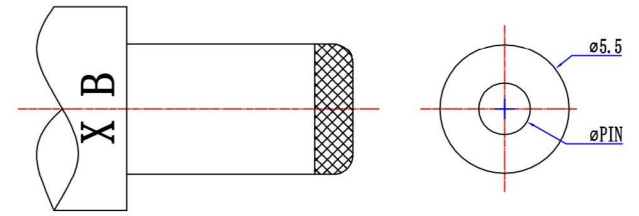
DC MATE PLUG
