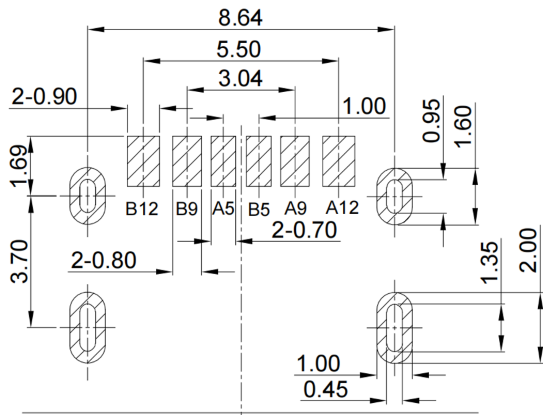
RECOMMENDED P.C.B. LAYOUT TOLERANCE UNSPECIFIED ±0.05mm
