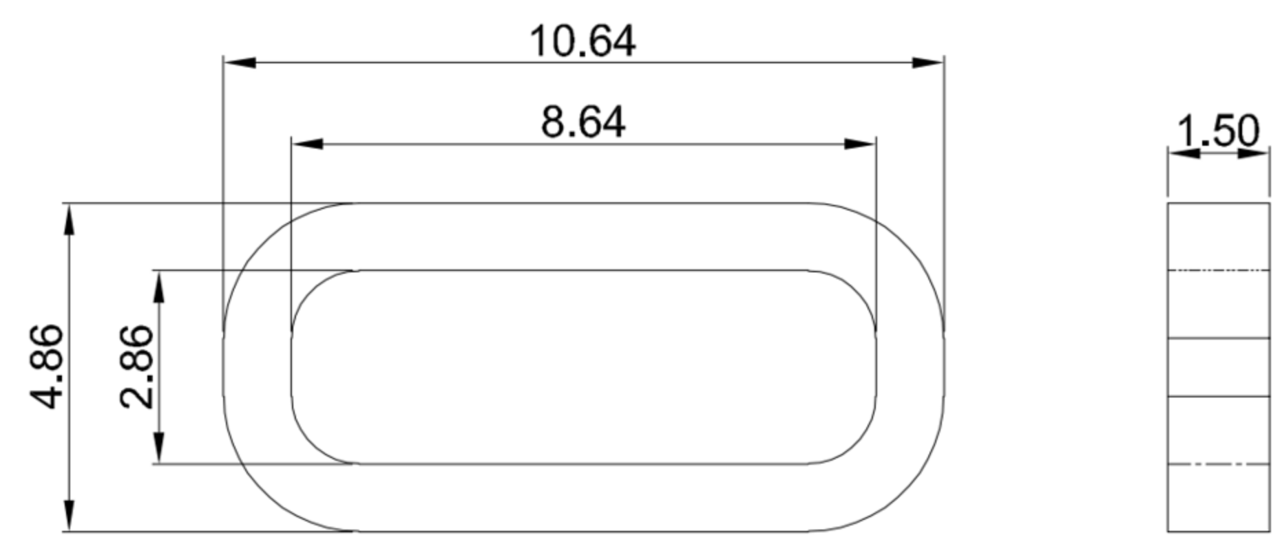
SUGGESTED RUBBER RING SIZE
