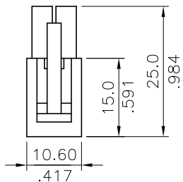
4 CIRCUITS (P/N: CP1104S000A)
