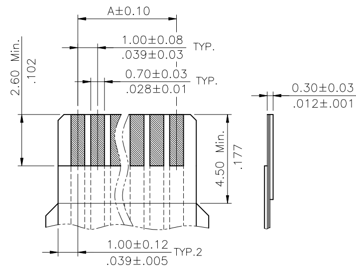
Accommodated FPC
