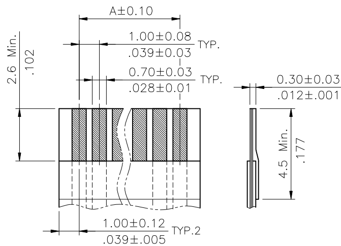
Accommodated FFC
