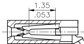
SEC.: X-X
