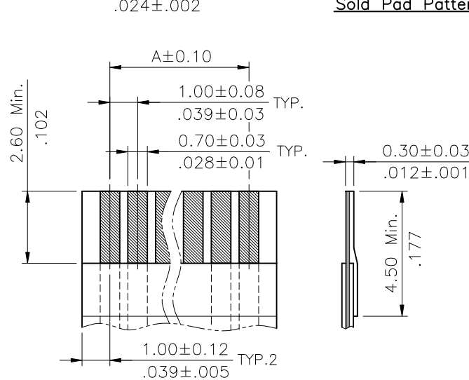
Accommodated FFC
