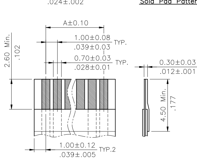
Accommodated FFC
