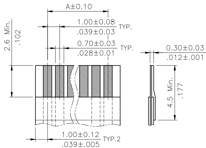
Accommodated FFC
