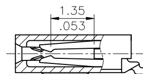
SEC.: X-X
