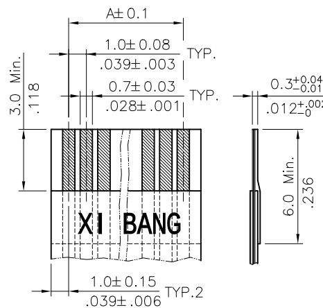
Accommodated FFC
