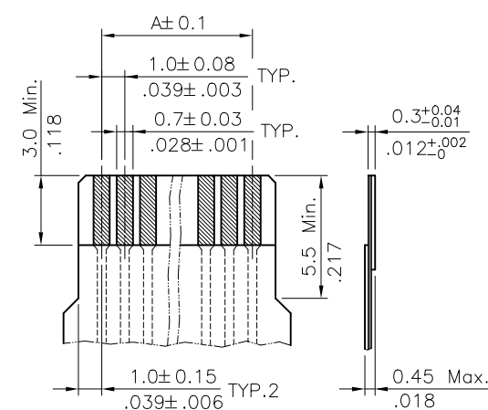
Accommodated FPC
