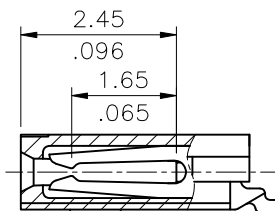
SEC.: Y-Y
