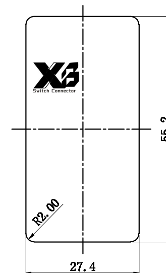
PANEL CUT-OUT
