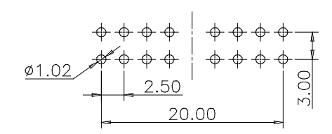
Recommended P.C.Board Layout (Tolerance:±0.05)
