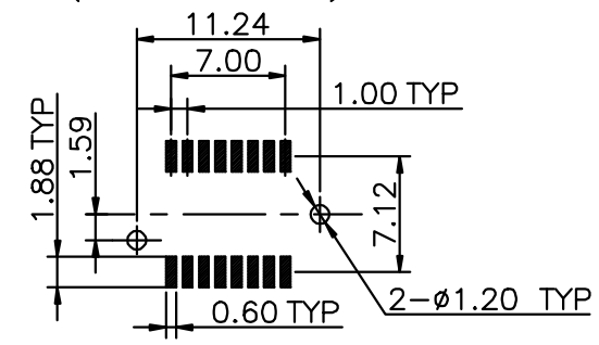
Recommended P.C.Board Layout (Tolerance:±0.05)
