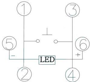
SCHEMATIC (SHORTING)
