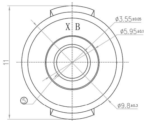
Matching Plug
