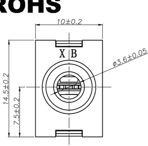
MATE PLUG
