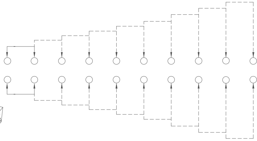
SCHEMATIC (NON-SHORTING)
