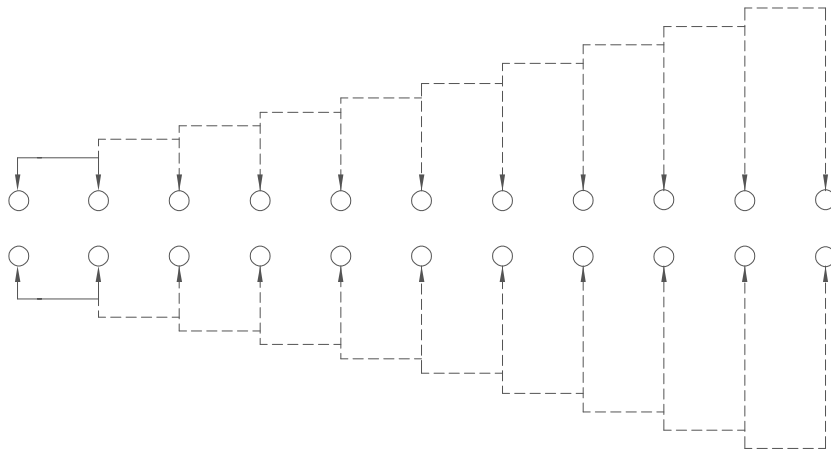
SCHEMATIC (NON-SHORTING)
