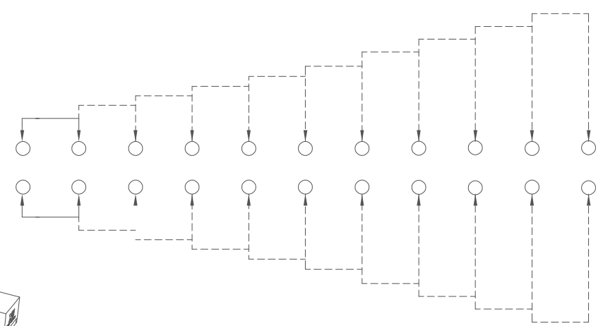
SCHEMATIC (NON-SHORTING)
