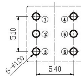
P.C.B INSTALLATION DIAGRAM
