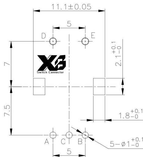
P. C. B MOUNTING HOLE DETAIL
