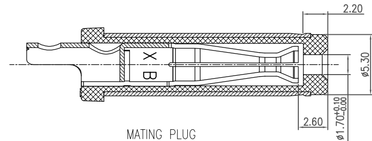
MATING PLUG DP550170-0192-60000H
