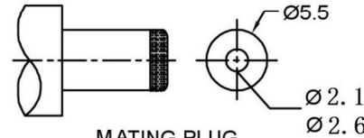
MATING PLUG
