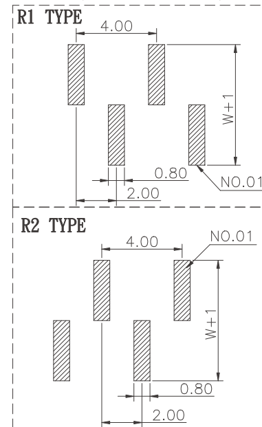
Recommended P.C.Board Layout (Tolerance:±0.05)
