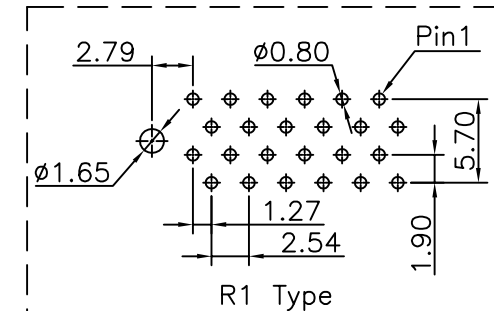
Recommended P.C.Board Layout (Tolerance:±0.05)
