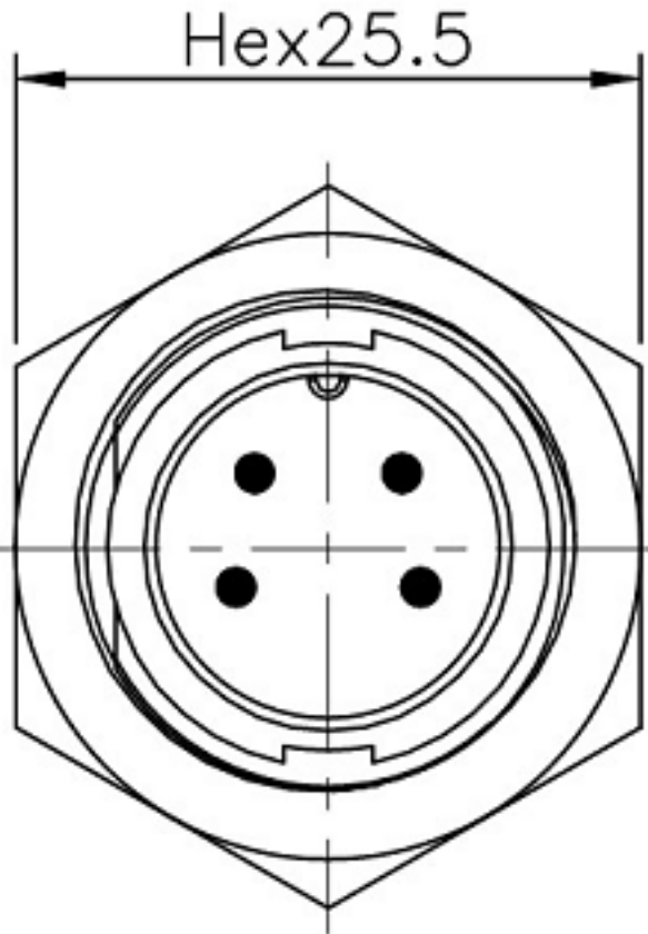
Assembly View
