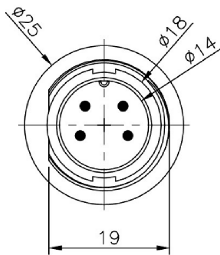
Body
