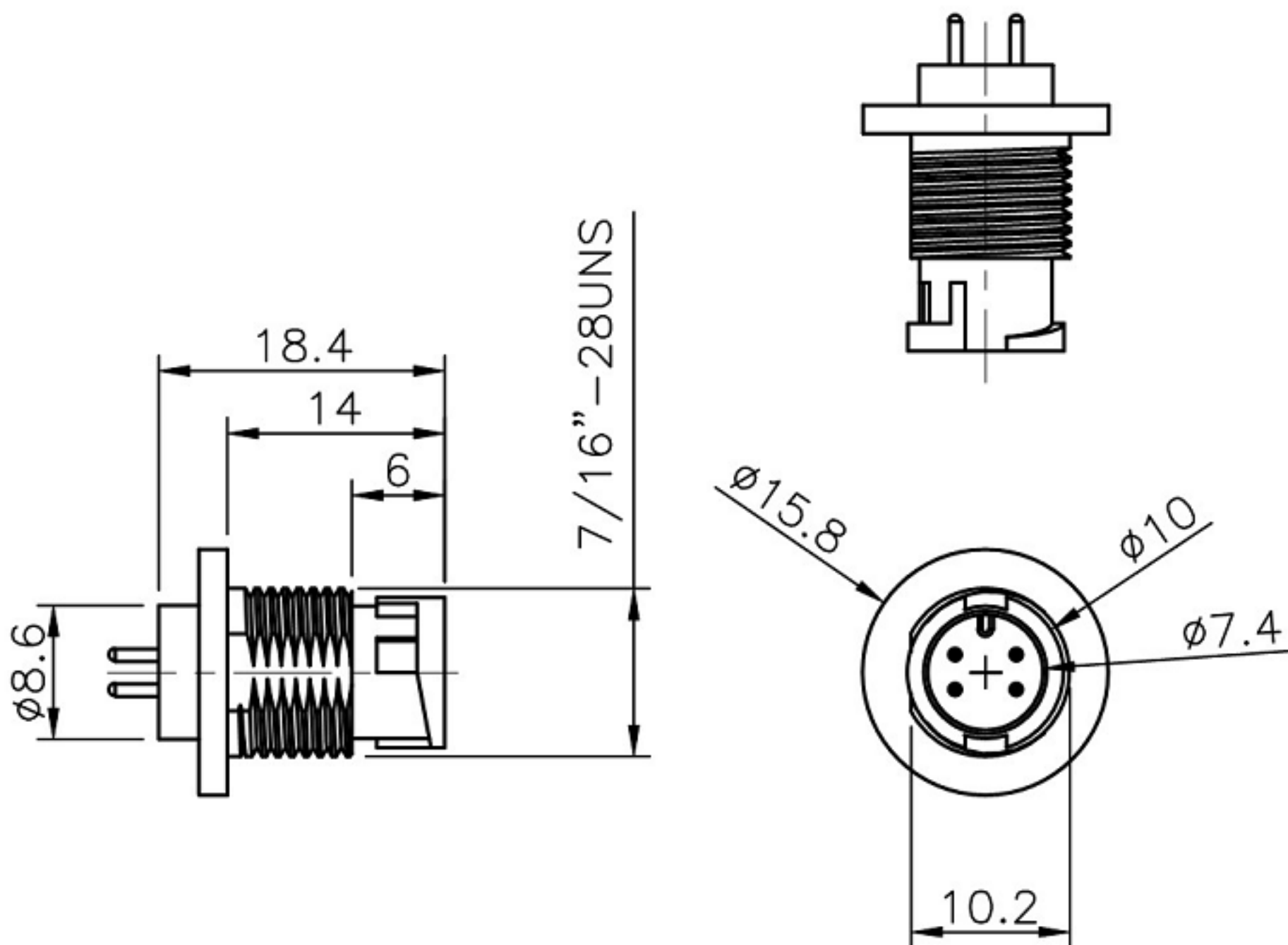
Body
