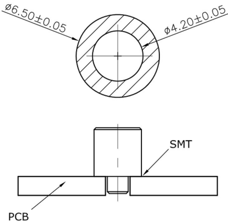
PCB Recommend Layout Pattern
