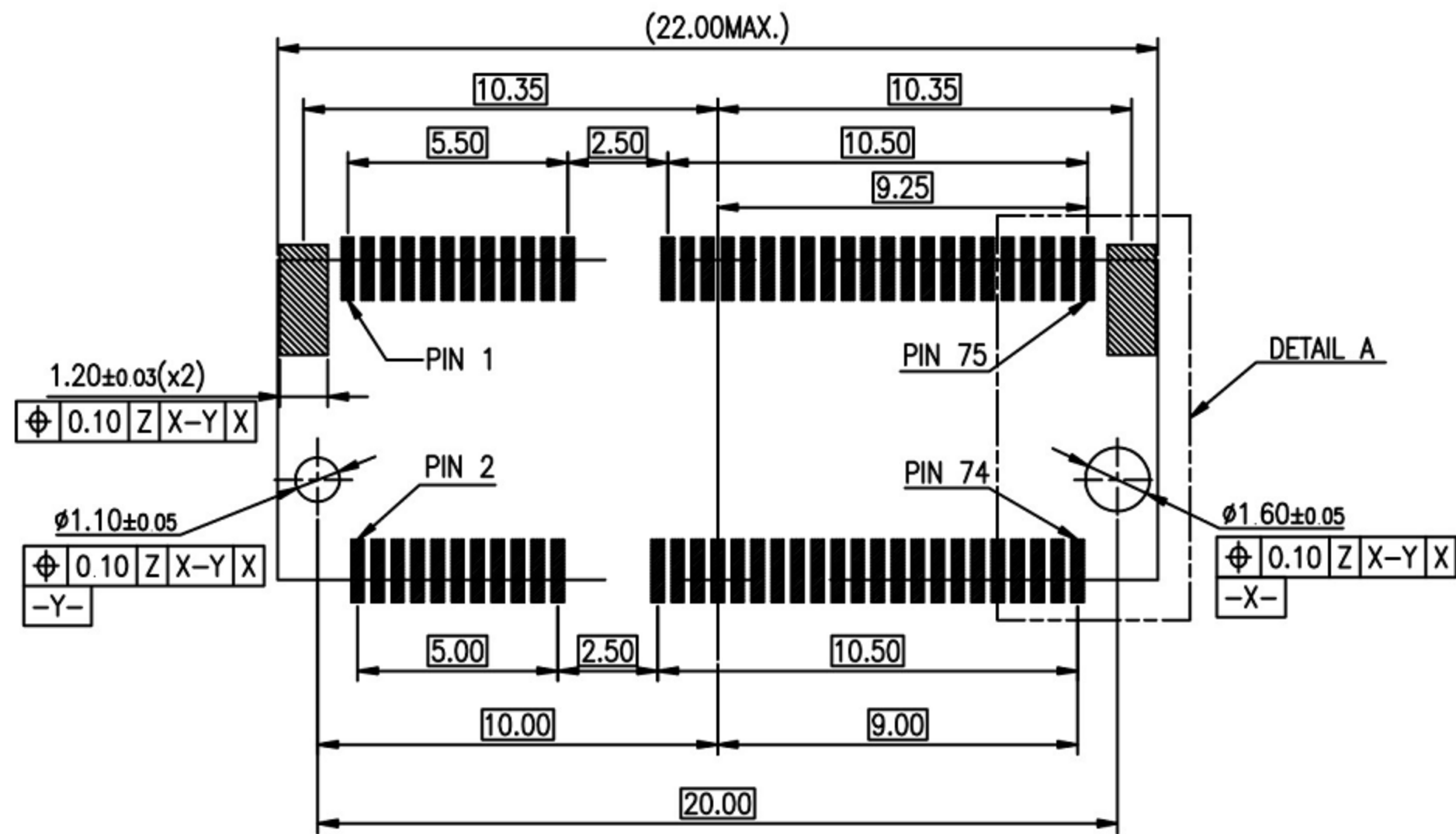
RECOMMEND PCB LAYOUT(TOP VIEW) (DEFAULT TOLERANCE:±0.05mm)
