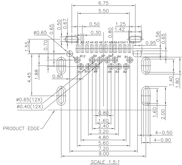
SCALE 1.5:1 RECOMMENDED PCB LAYOUT(TOP VIEW) THICKNESS 1.0 MM;DEFAULT TOLERANCE:±0.05
