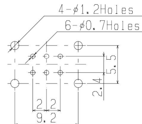
PC board mounting hole dimension (TOP VIEW)
