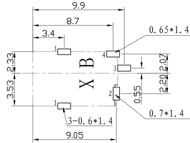
PCB LAYOUT
