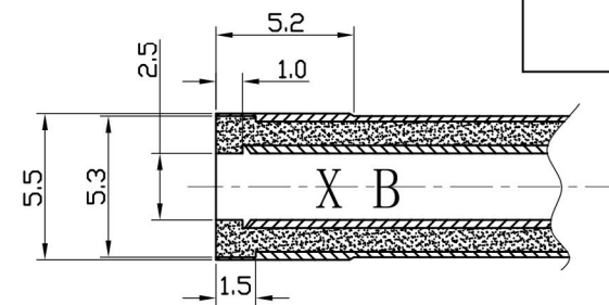
MATING PLUG
