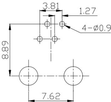
RECOMMENDED P.C.B LAYOUT TOP VIEW (COMPONENT SIDE)
