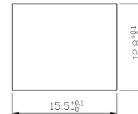
Mounting Panel Hole Dimensions
