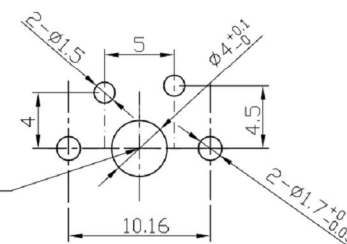
P.C.B. Mounting Hole Dimensions
