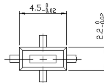
DETAIL C 2/1
