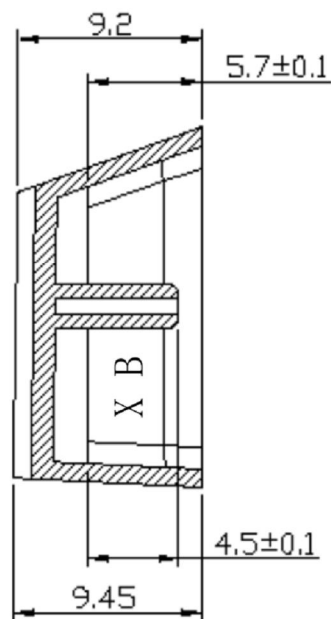
SECTION B-B
