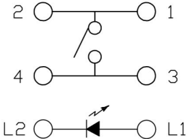
ELECTRICAL DIAGRAM
