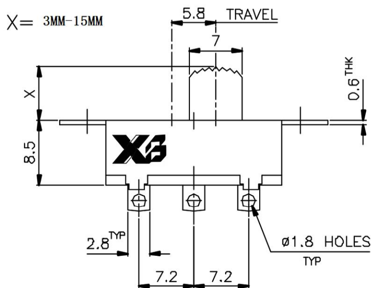
SLIDE SWITCH 2P2T
