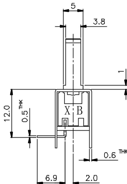
SLIDE SWITCH 1P3T
