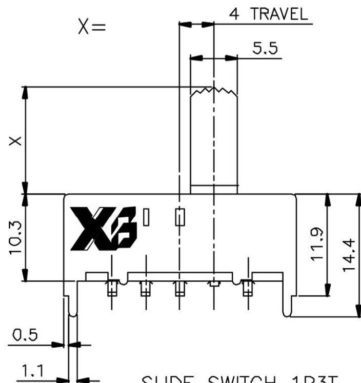
SLIDE SWITCH 1P3T
