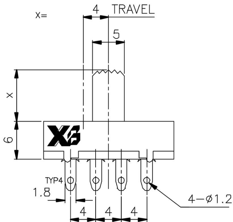
SLIDE SWITCH 1P3T
