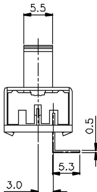
SLIDE SWITCH 1P3T
