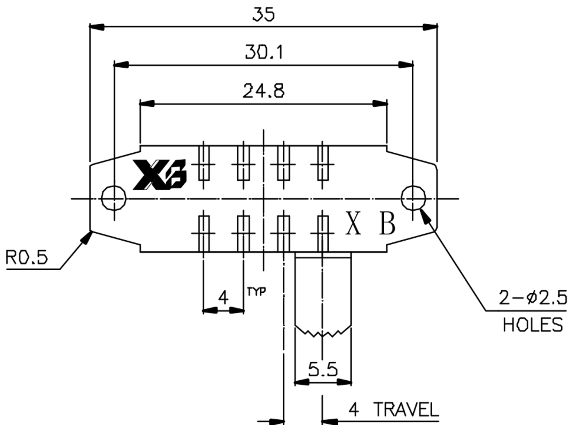
SIDE KNOB SLIDE SWITCH 2P4T
