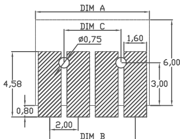
RECOMMENDED PCB LAYOUT TOL (<math>\pm 0.05</math>)
