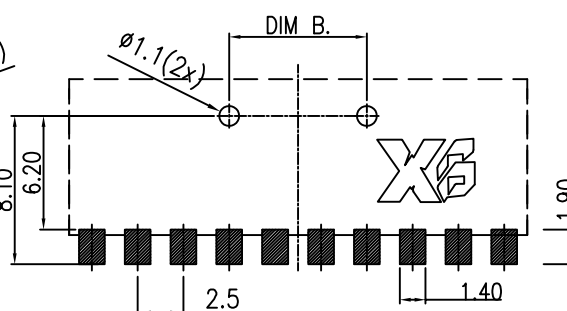
RECOMMENDED P.C.B LAYOUT TOP VIEW (TOLRANCE:±0.05)
